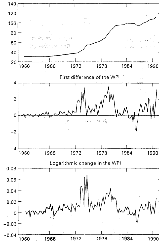
Figure 2.5 U.S. wholesale price index (1985 = 100).
