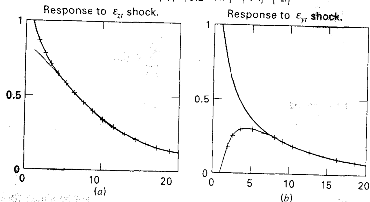
Figure 5.6 Two impulse response functions.
