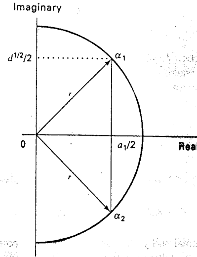
Figure 1.6 Characteristic roots and the unit circle.
