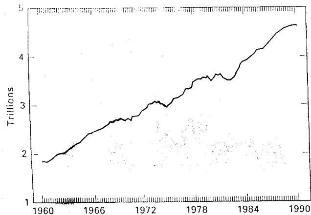
Figure 3.1 U.S. GNP (1985 price).
