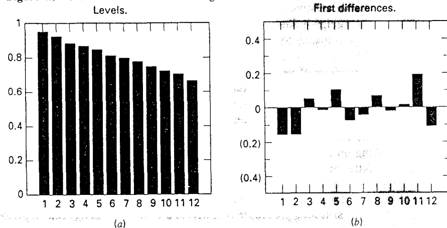
Figure 4.3 ACF of Canada's real exchange rate.
