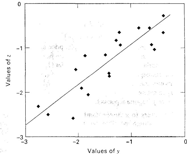
Figure 6.1 Scatter plot of cointegrated variables.
