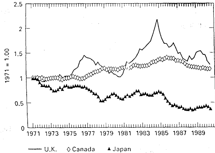
Figure 3.7 Exchange rate indices (currency/dollar).
