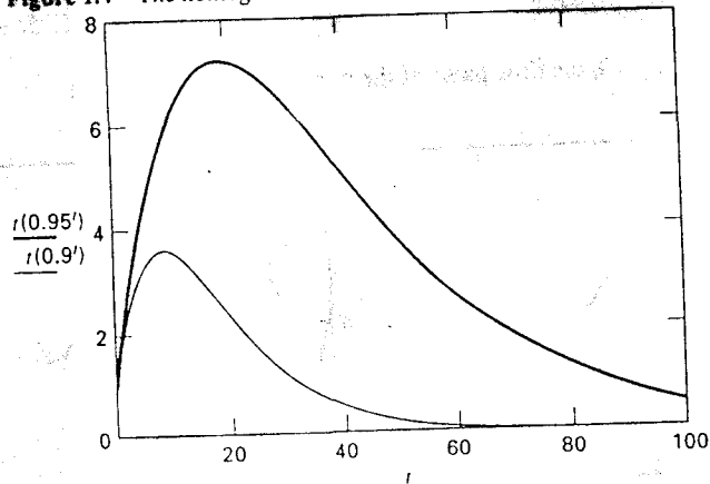
Figure 1.4 The homogeneous solution t \cdot (a_1)^t .
